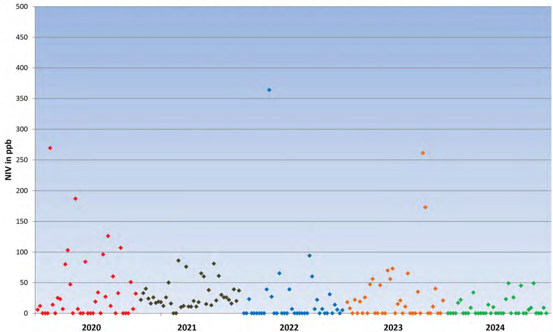
NIV \mu\text{g/kg} in UK Barley from crop years 2020 to 2024
