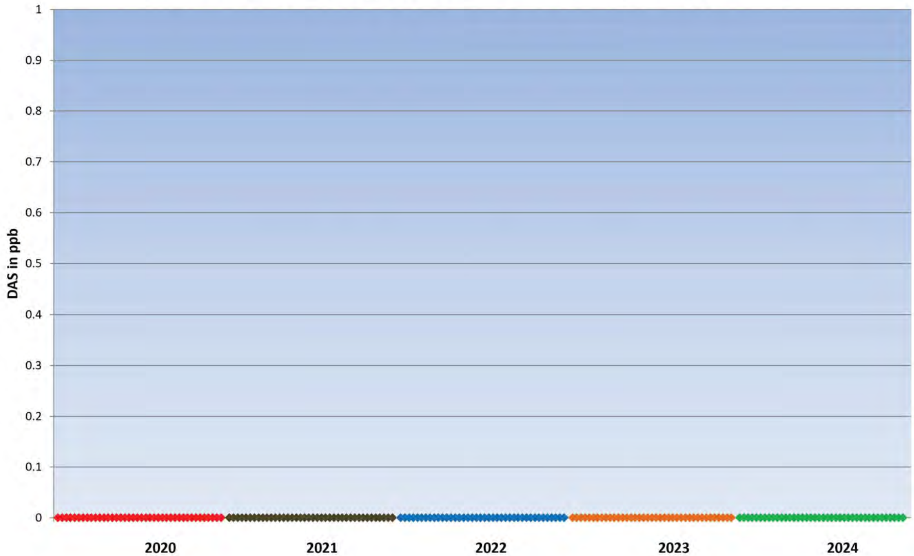
Diacetoxyscirpenol (DAS) \mu\text{g}/\text{kg} in UK Barley from 2020 to 2024 crop years
