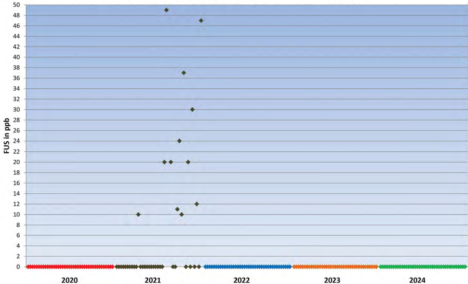
Fusarenone-X (FUS) µg/kg in UK Barley from 2020 to 2024 crop years
