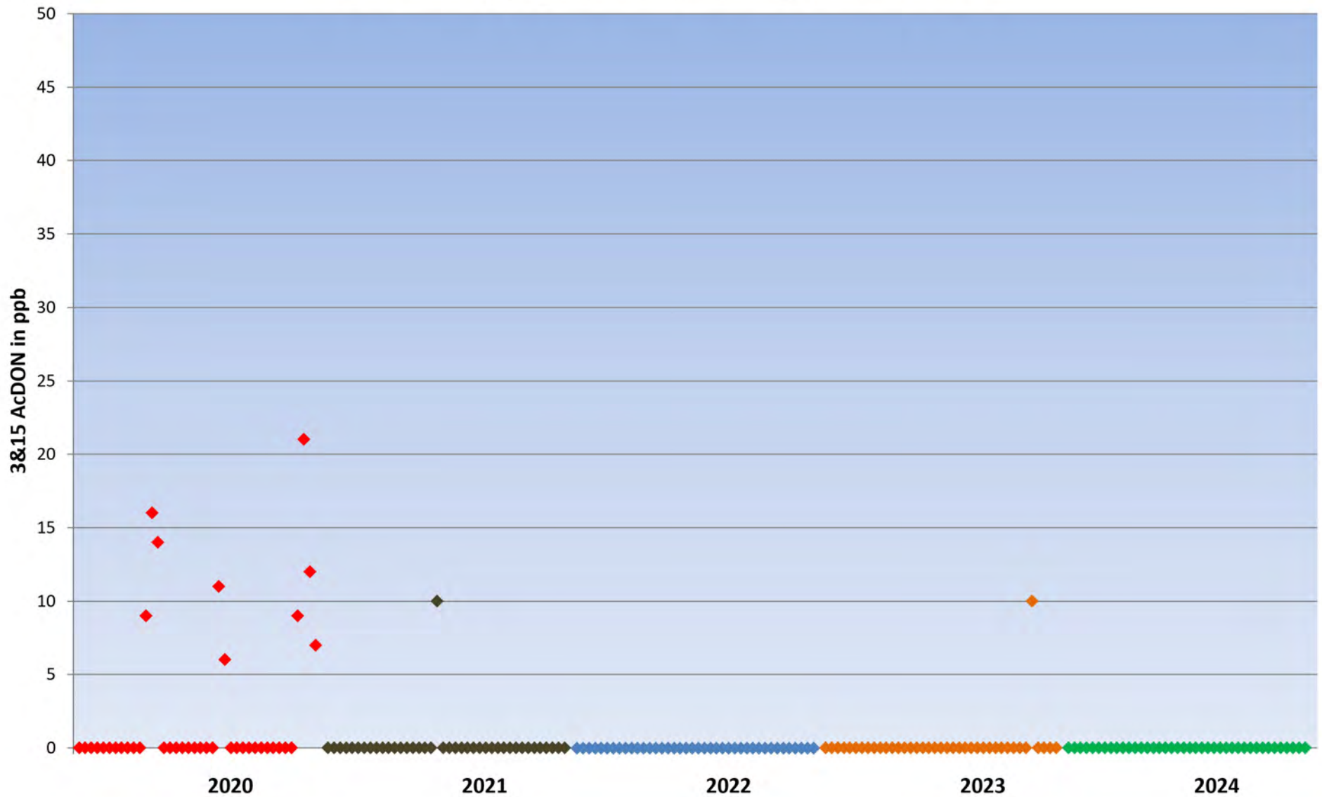
3 & 15-AcDON \mu\text{g/kg} in UK Barley from crop years 2020 to 2024
