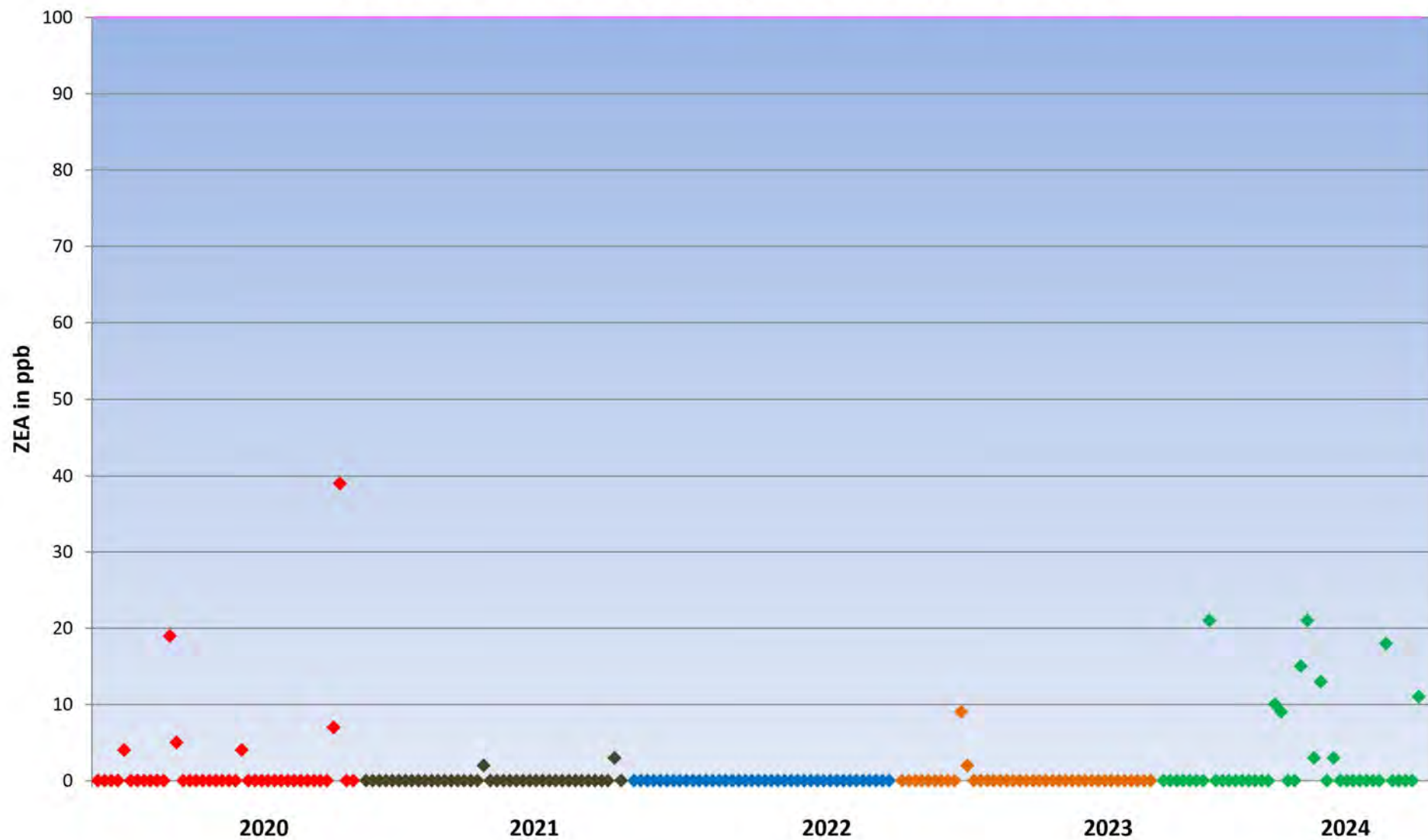
Zearalenone \mu\text{g}/\text{kg} in UK Barley from 2020 to 2024 crop years. (EU MRL was set at 100 ppb ( \mu\text{g}/\text{kg} ) in unprocessed cereals in 2007)
