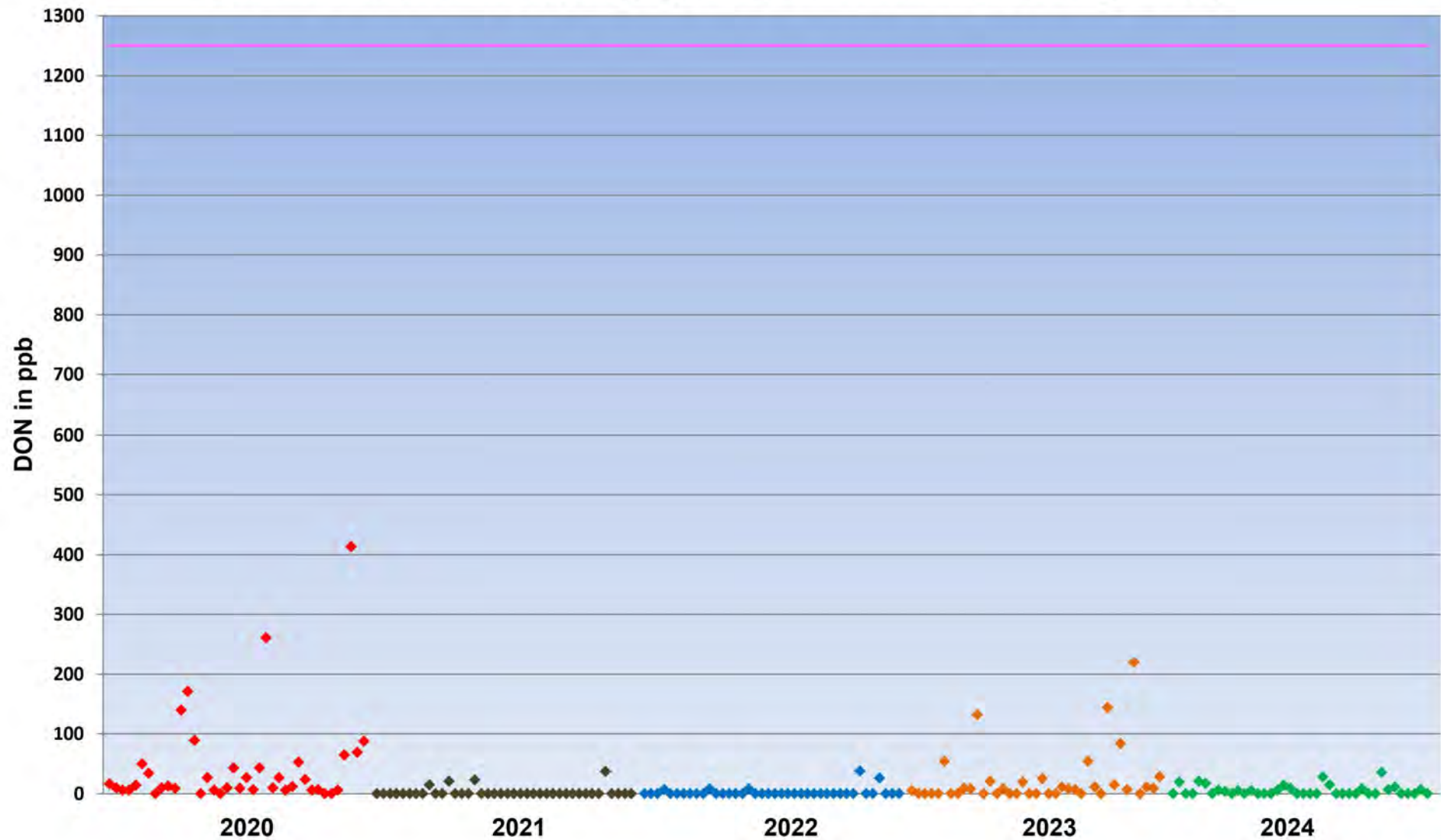
DON \mu\text{g}/\text{kg} in UK Barley from crop years 2020 to 2024 (EU MRL was set at 1250ppb ( \mu\text{g}/\text{kg} ) for DON in cereals for processing in 2007)
