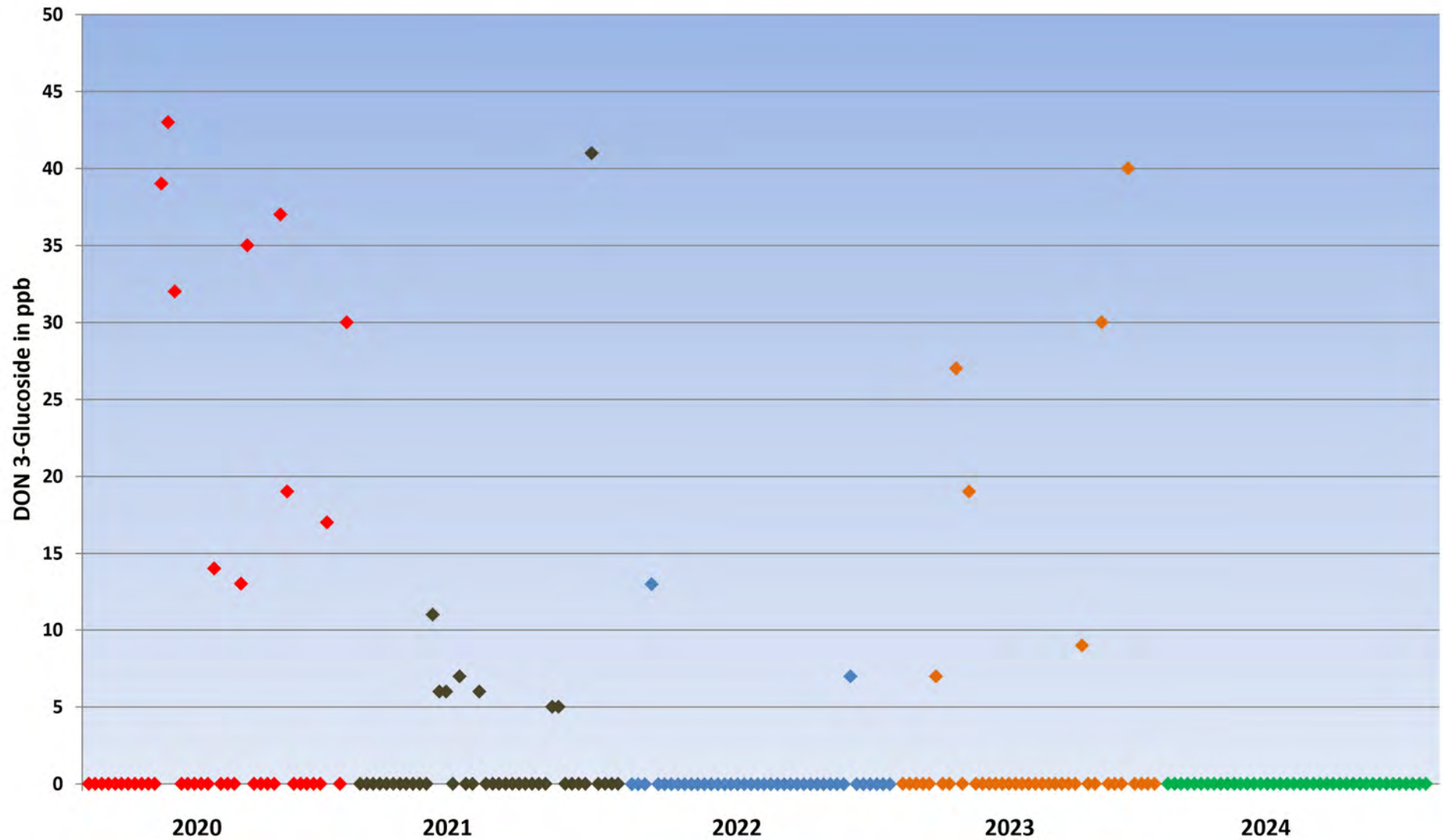
DON 3-Glucoside µg/kg in UK Barley from crop years 2020 to 2024
