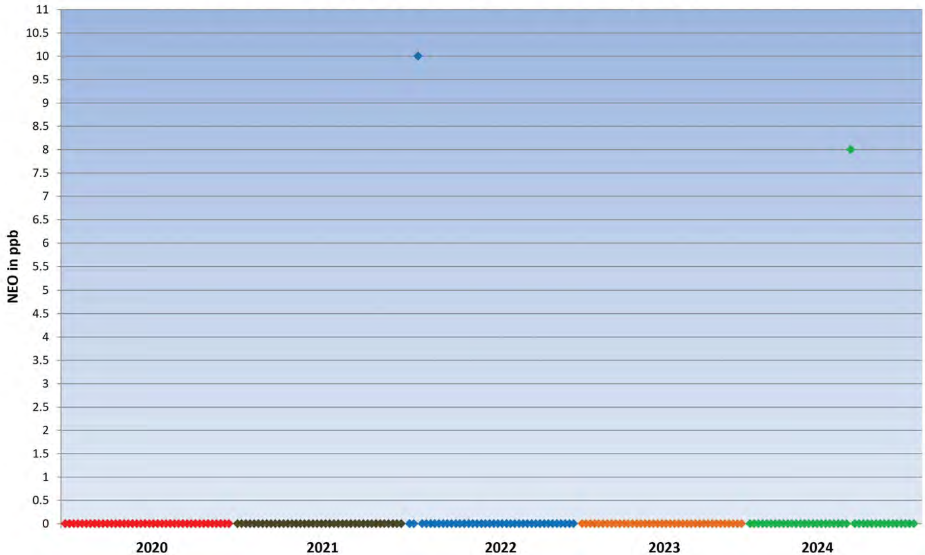
Neosolaniol (NEO) \mu\text{g}/\text{kg} in UK Barley from 2020 to 2024 crop years
