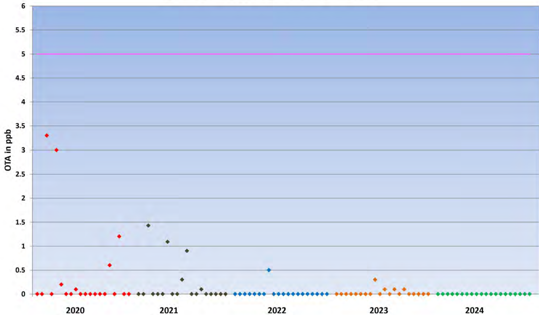
OTA µg/kg in UK Barley from crop years 2020 to 2024 (EU MRL set at 5ppb (µg/kg) in barley from 2003)
